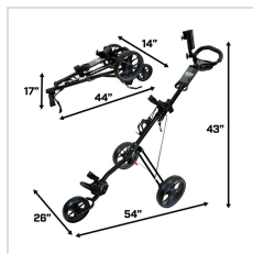
Dimensions (A99933)
